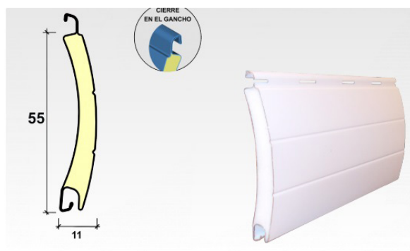
Curved profile aluminium slat with polyurethane Slat of 55-C mm.
