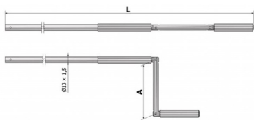
Complete Articulated Crank Handle D13 A180 L1500
