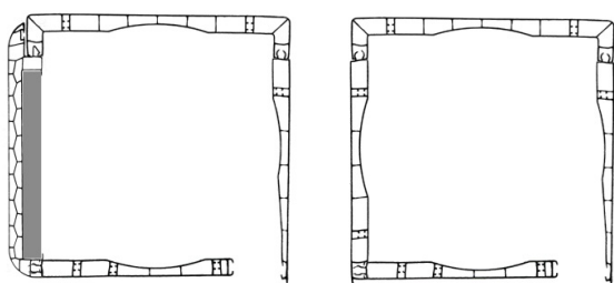
PVC Box - Decorative with insulation 155,185,200, 225 mm
