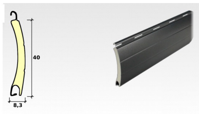
Curved profile aluminium slat with polyurethane Slat of 40-C mm.
