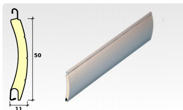
Curved profile aluminium slat with polyurethane Slat of 50 mm.
