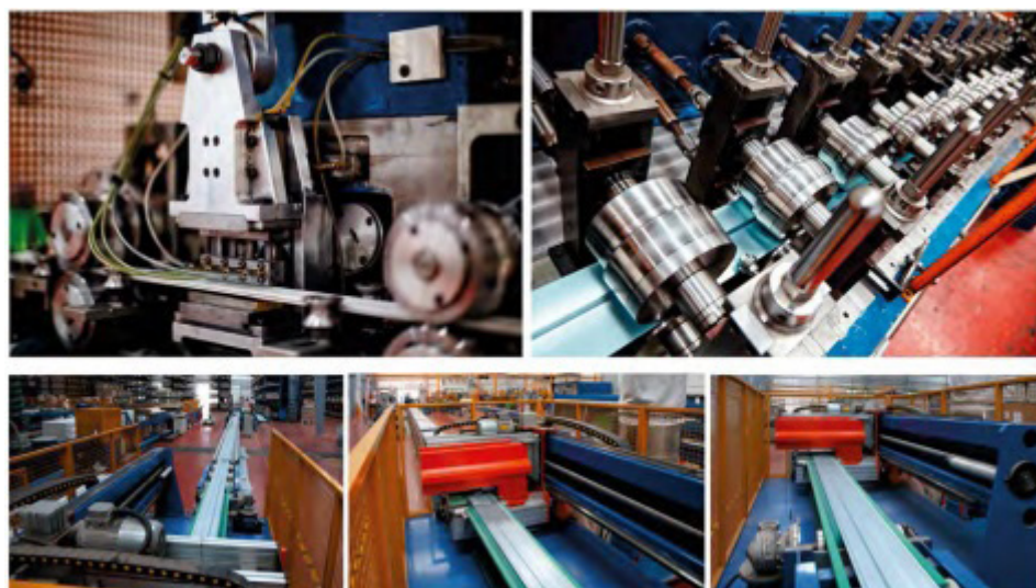
Aluminium box with polyurethane “aislaBoxUltra” roll forming machines.
