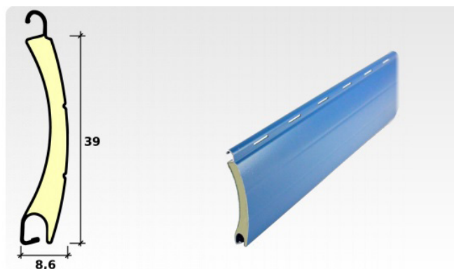
Curved profile aluminium slat with polyurethane Slat of 39 mm.
