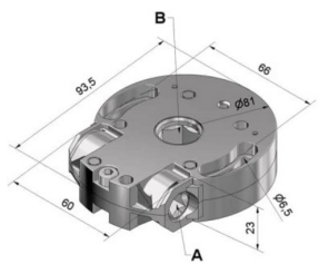
Cardan Mechanism Kg SINFIN R7:1 C8 HEX16 CON FIN
