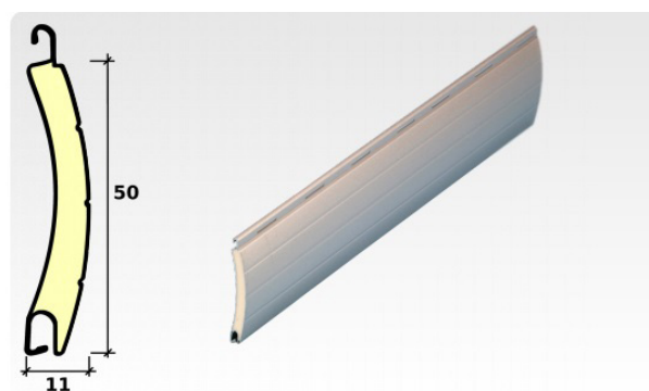
Curved profile aluminium slat with polyurethane Slat of 50 Plus mm.
