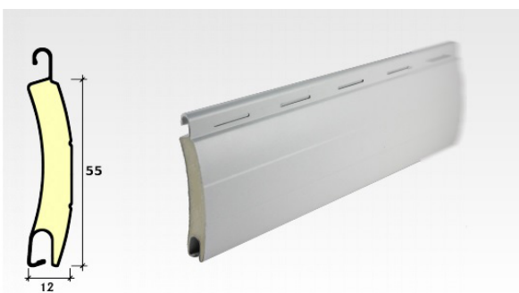
Curved profile aluminium slat with polyurethane Slat of 55I Plus mm.
