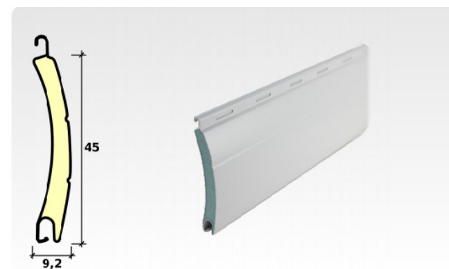
Curved profile aluminium slat with polyurethane Slat of 45 mm.
