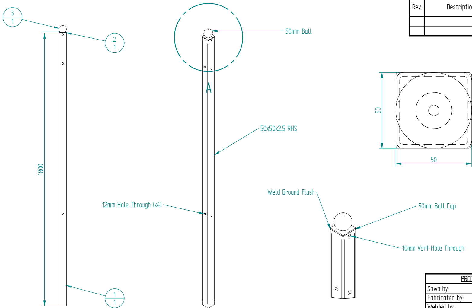
DETAIL A
