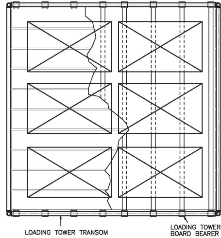
Six No. 0.85kN (0.85 Ton) Pallets
