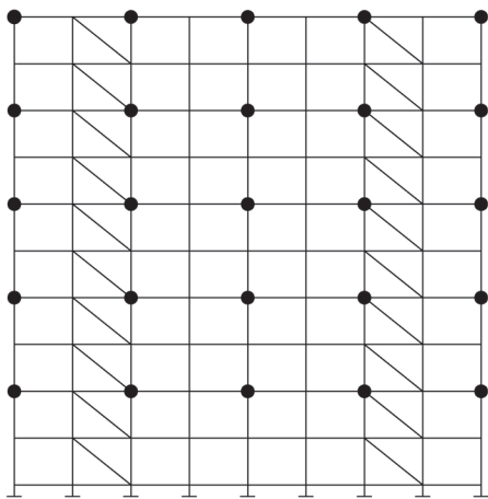
(A) Lines of Ties on Alternate Lifts
