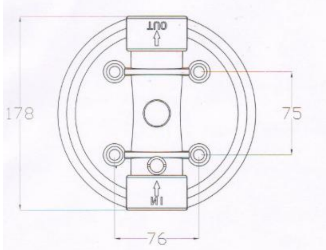
BIG BLUE FILTER HOUSING 10 INCH 1" PORTS WITH BRASS INSERTS
